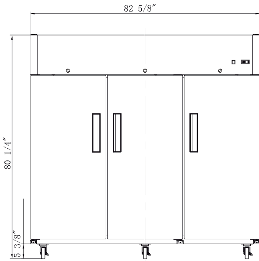
Front View
