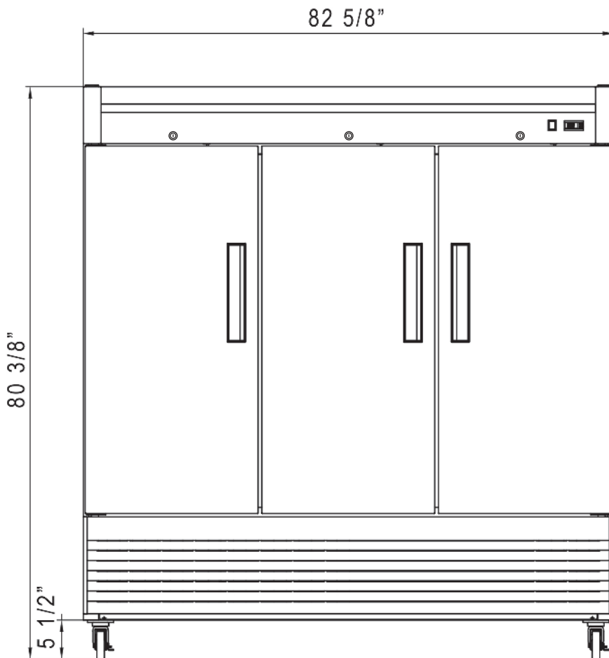
Front View
