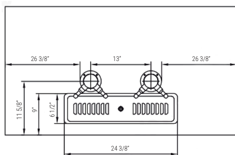
Keg configuration
