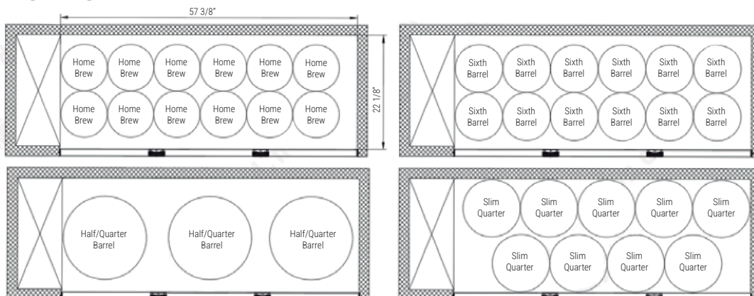
Keg configuration
